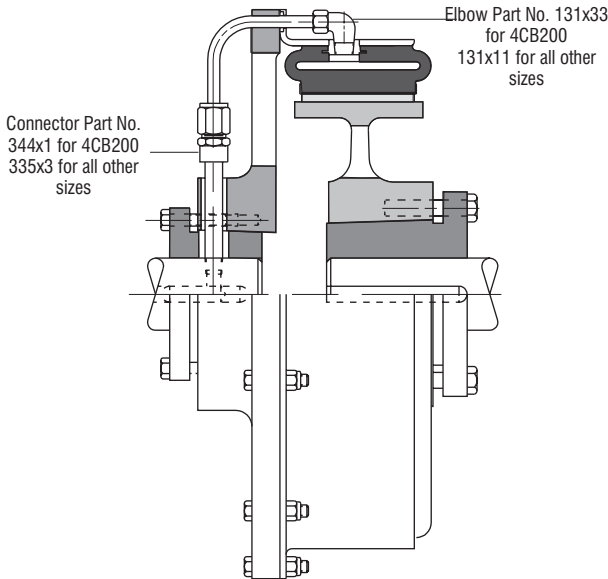
PCB - 206 Arrangement
