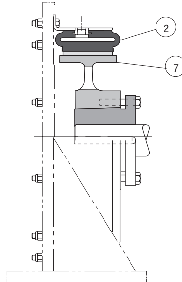
PCB - 208 Arrangement
